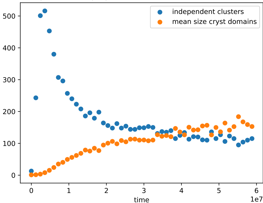
Crystallisation properties, PVA-100, T = 0.88 , \dot{T} = 10^{-3}
