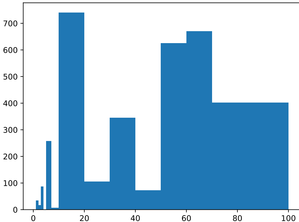
Crystalline domain size distribution, PVA-100, time 12000000, \phi = 0.366
