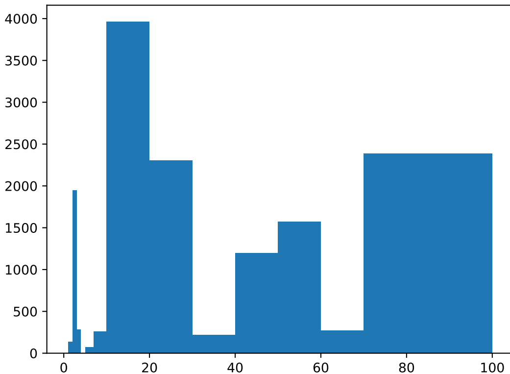
Crystalline domain size distribution, PVA-100, time 120000000, \phi = 0.486
