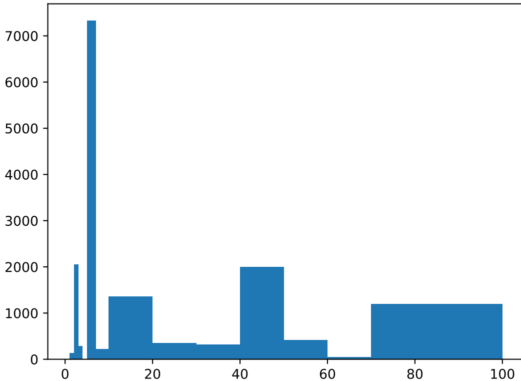
Crystalline domain size distribution, PVA-100, time 144000000, \phi = 0.491
