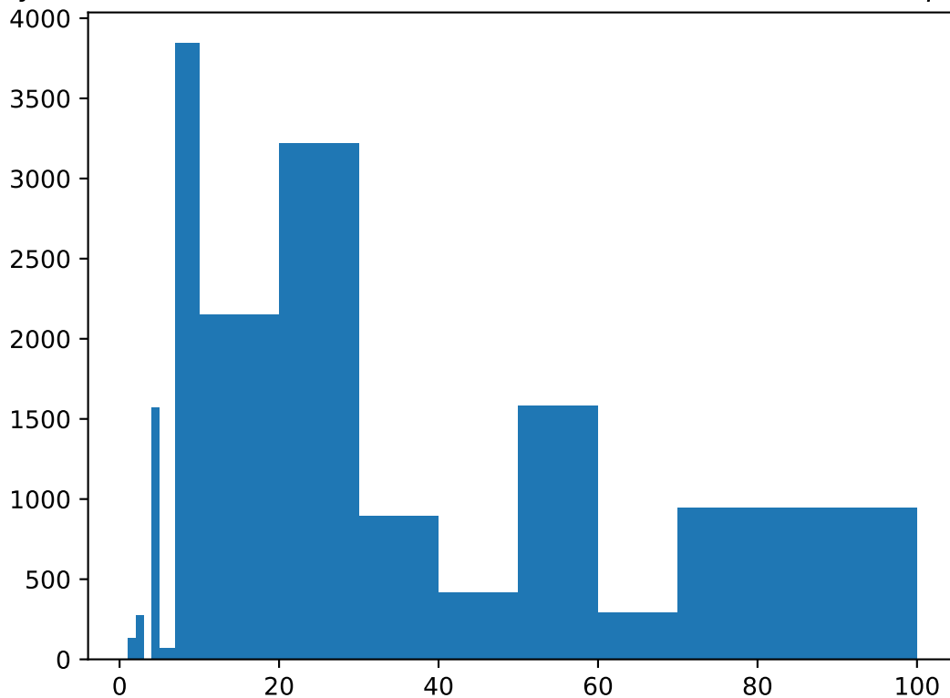
Crystalline domain size distribution, PVA-100, time 145200000, \phi = 0.492
