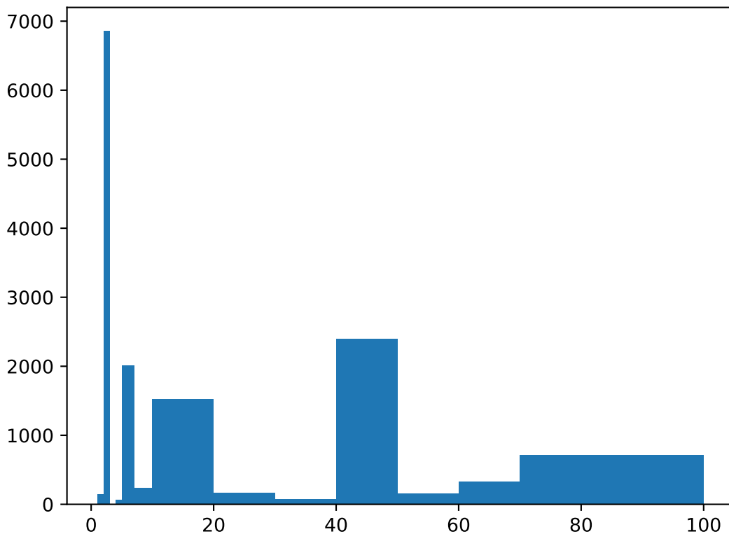
Crystalline domain size distribution, PVA-100, time 156000000, \phi = 0.493
