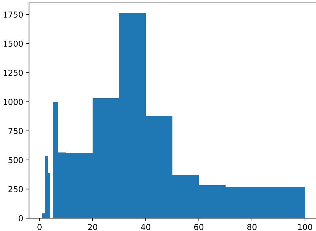
Crystalline domain size distribution, PVA-100, time 24000000, \phi = 0.417
