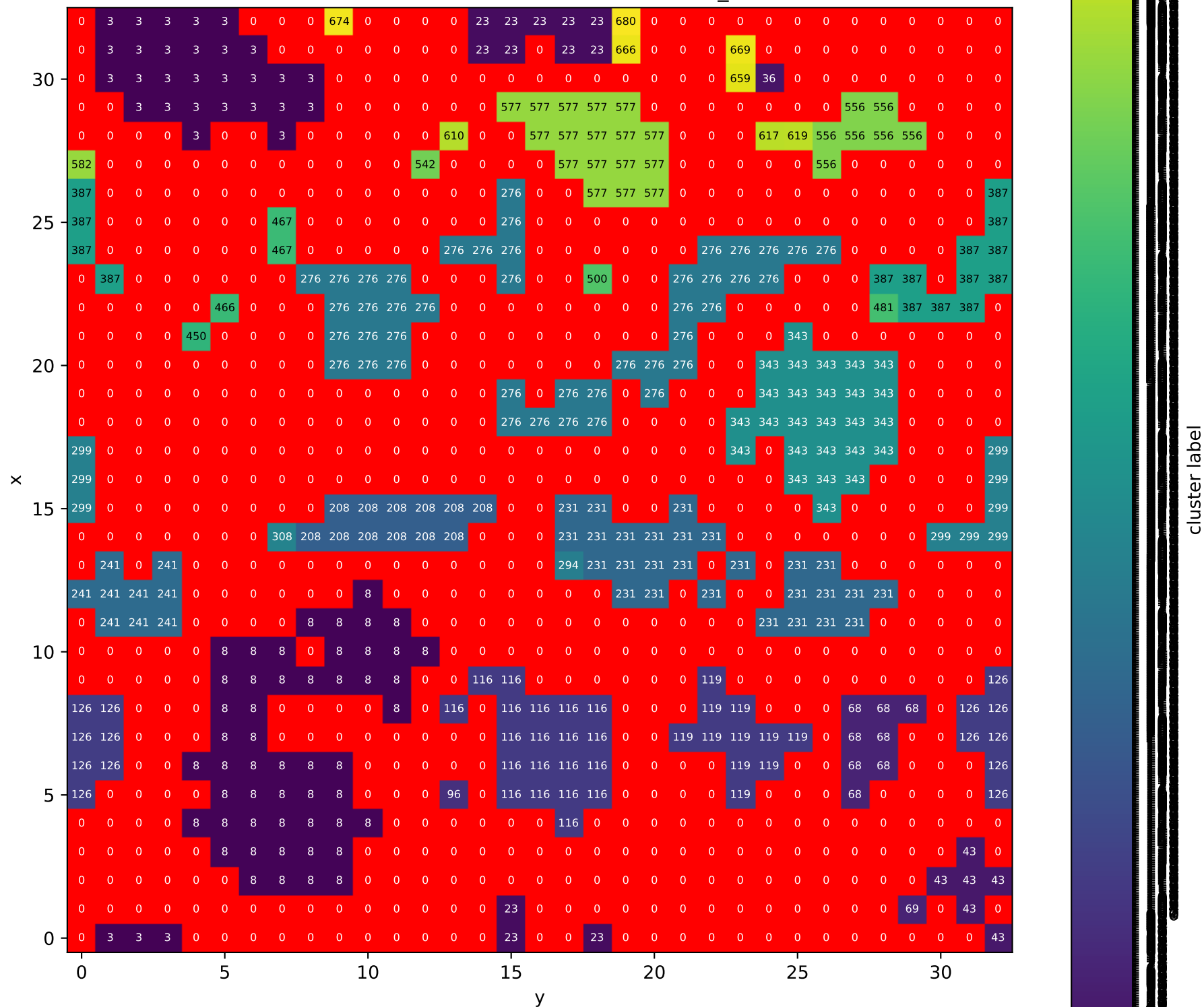
Cluster labels, PVA-100, T = 0.5, Tdot = 10**(-5), T_init = 1.0, z = 16
