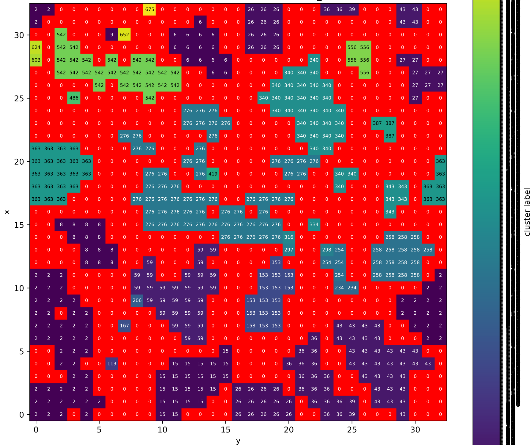
Cluster labels, PVA-100, T = 0.5, Tdot = 10**(-5), T_init = 1.0, z = 21
