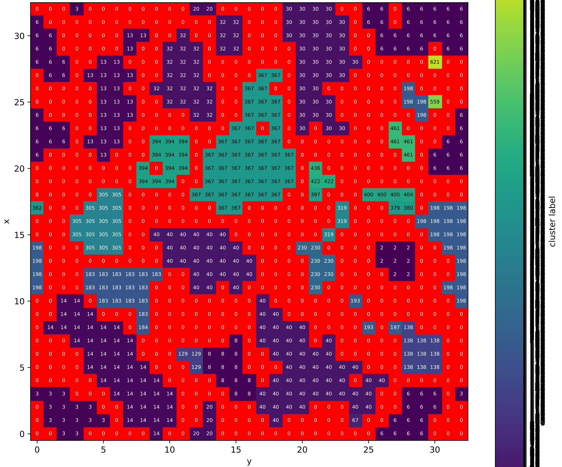
Cluster labels, PVA-100, T = 0.5 , T_{\text{dot}} = 10^{**}(-5) , T_{\text{init}} = 1.0 , z = 4
