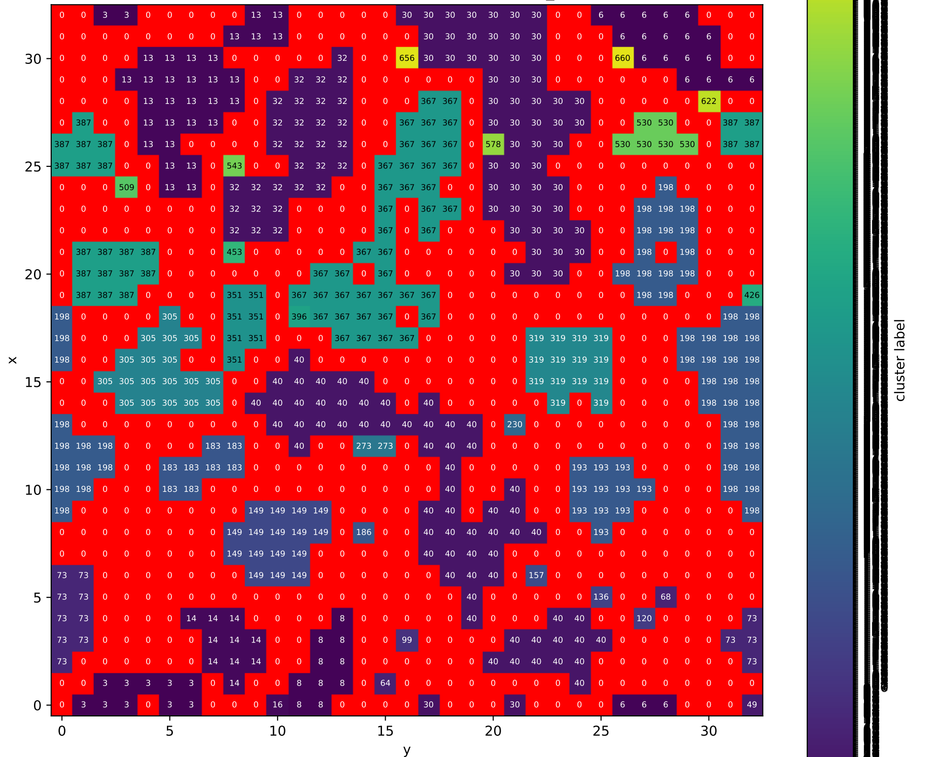
Cluster labels, PVA-100, T = 0.5, Tdot = 10**(-5), T_init = 1.0, z = 6
