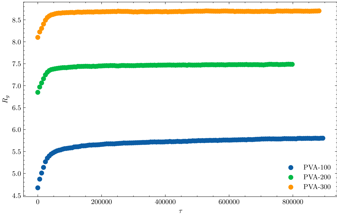
Mean gyration radius
