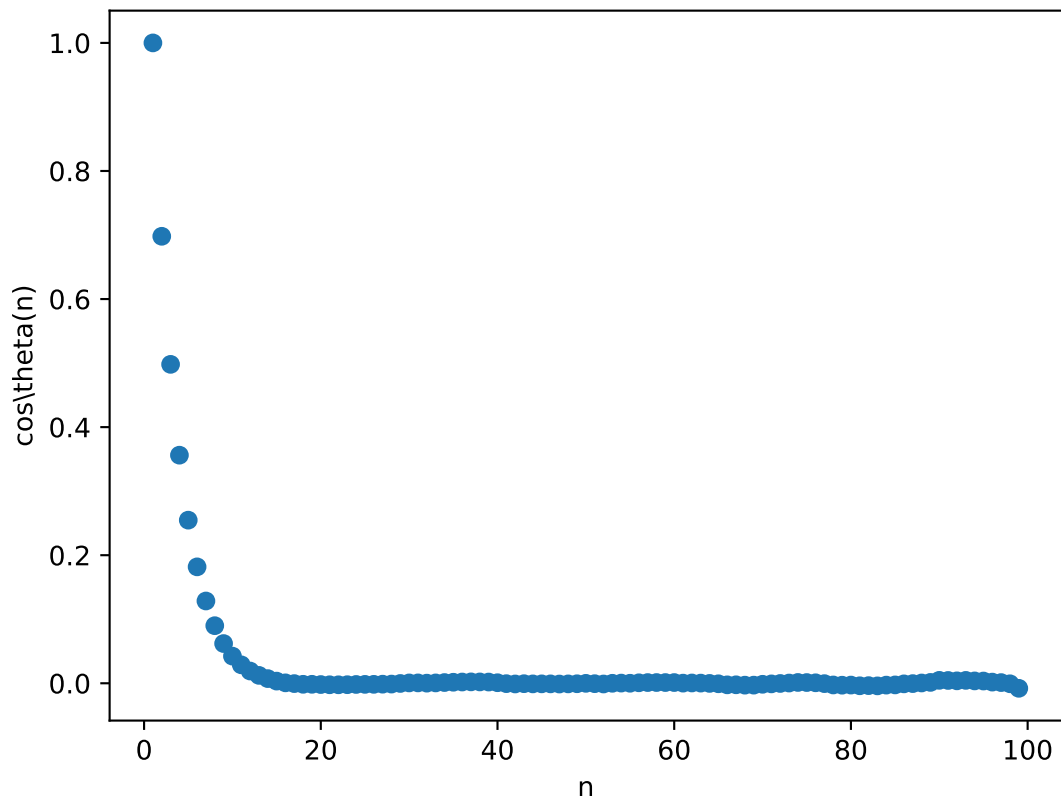
Distribution of bond-bond correlations, PVA-100
