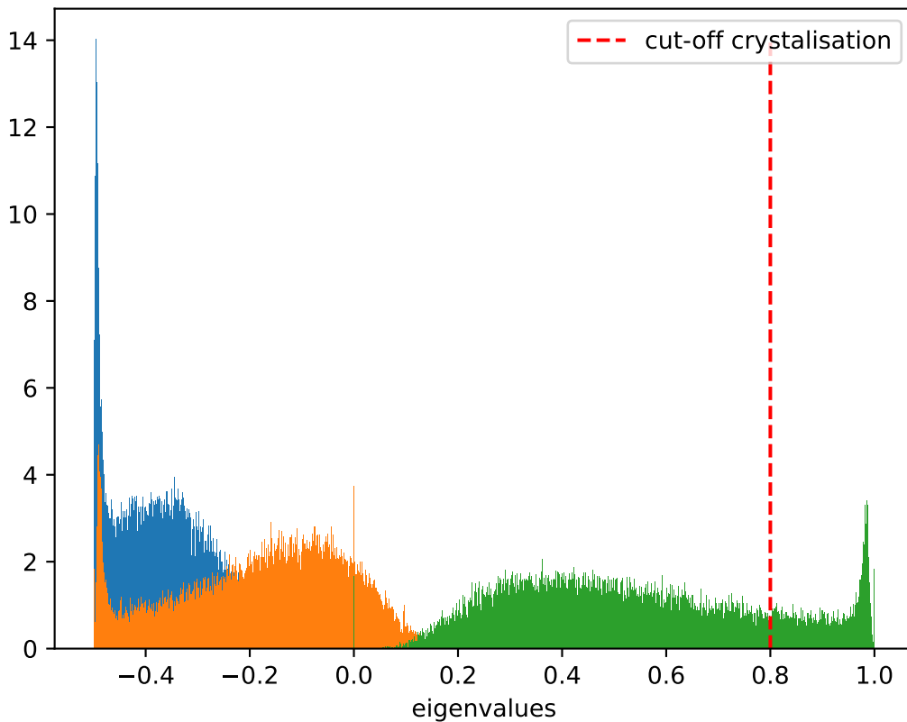
Distribution of eigenvalues at T = 0.675 , \dot{T} = 10^{-7}
