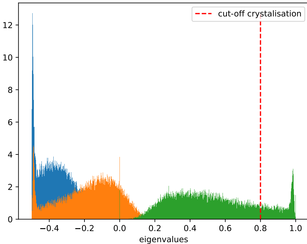
Distribution of eigenvalues at T = 0.7 , \dot{T} = 10^{-7}
