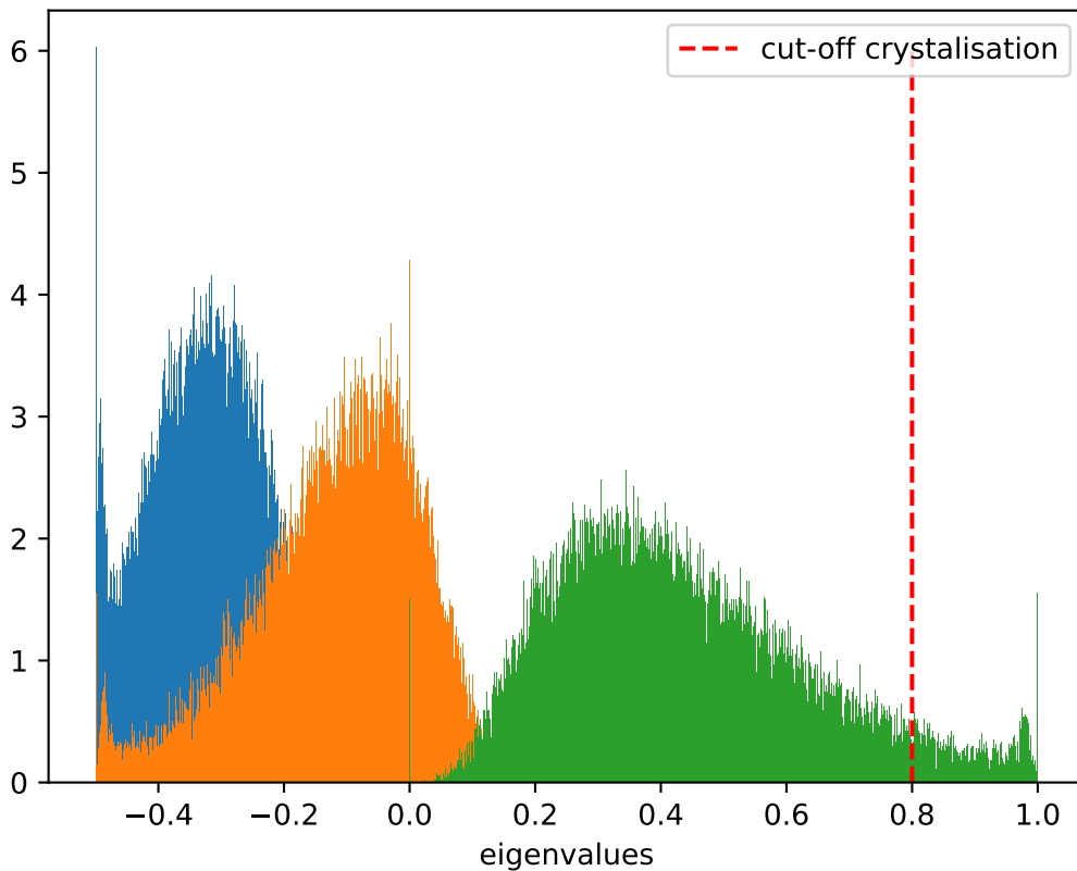
Distribution of eigenvalues at T = 0.825 , \dot{T} = 10^{-7}
