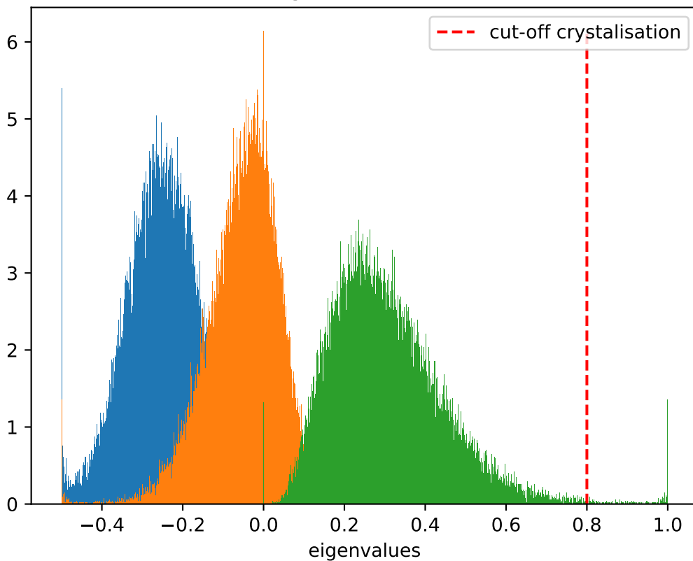
Distribution of eigenvalues at T = 1.0 , \dot{T} = 10^{-7}
