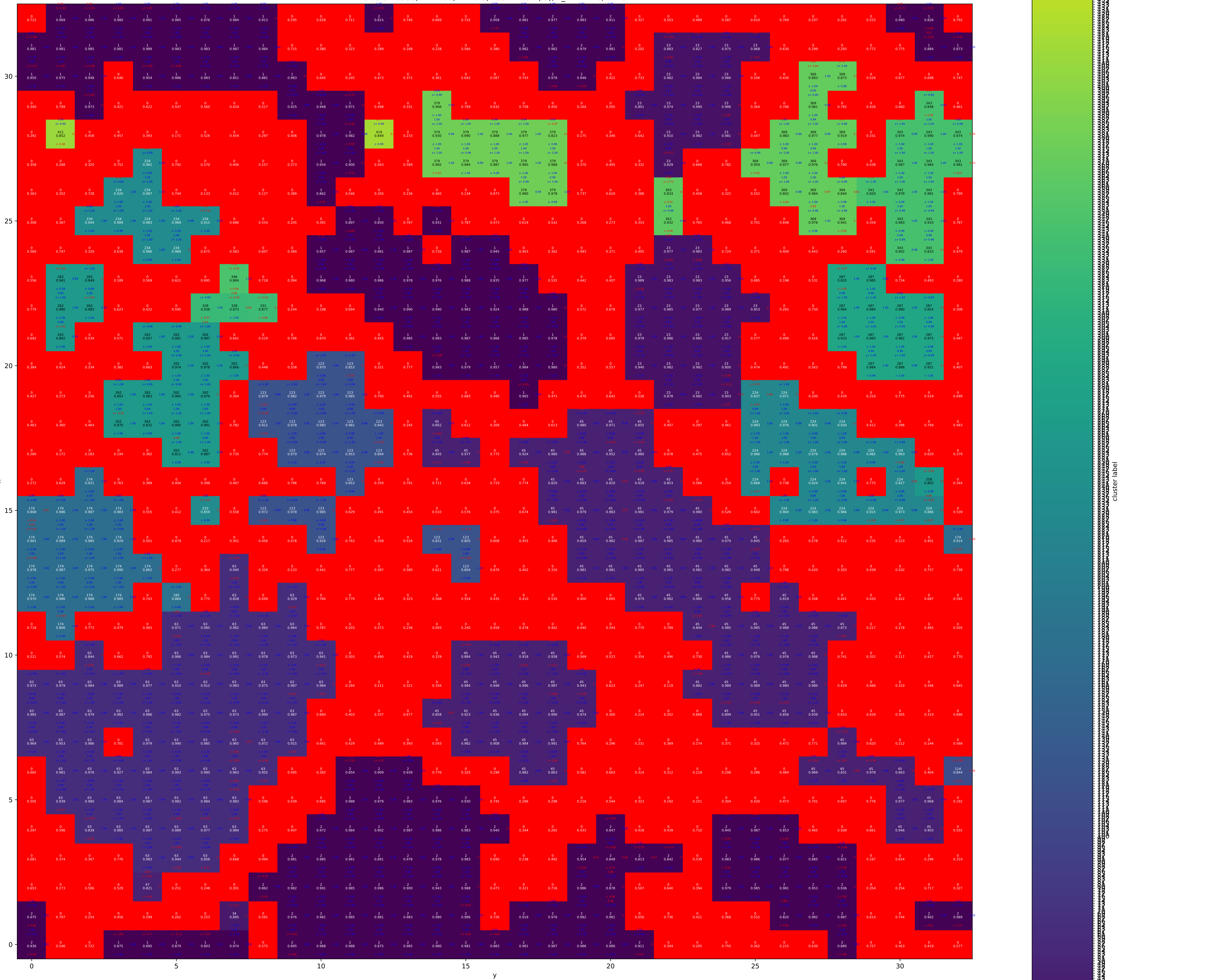
Cluster labels, PVA-100, T = 0.5, Tdot = 10**(-5), T_init = 1.0, z = 3
