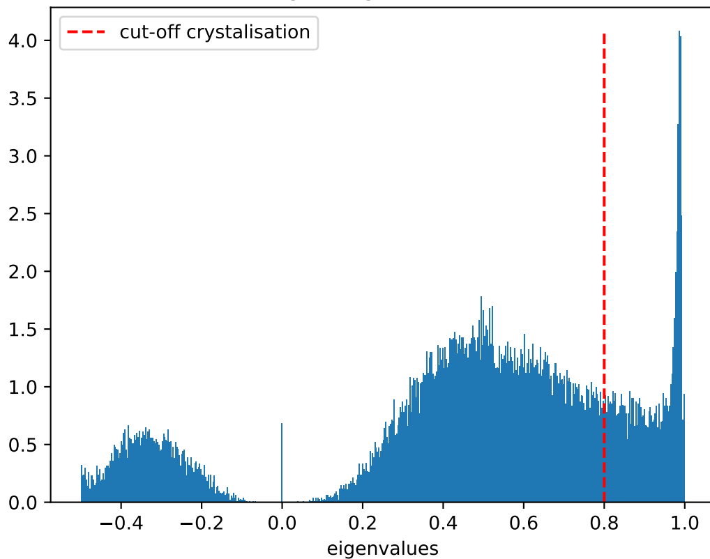
Distribution of largest eigenvalues, T = 0.5 , \dot{T} = 10^{-5}
