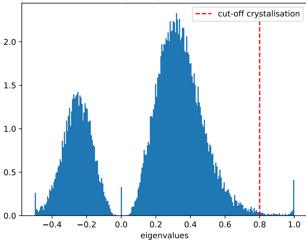
Distribution of largest eigenvalues, T = 1.0, \dot{T} = 10^{-5}
