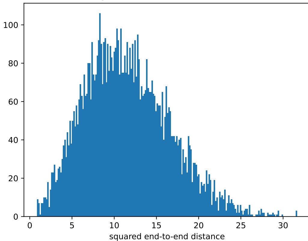
End-to-end length distribution, PVA-100, \dot{T} = 10^{-5} , T = 0.5
