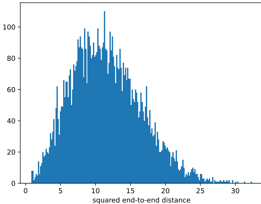
End-to-end length distribution, PVA-100, \dot{T} = 10^{-5} , T = 0.7
