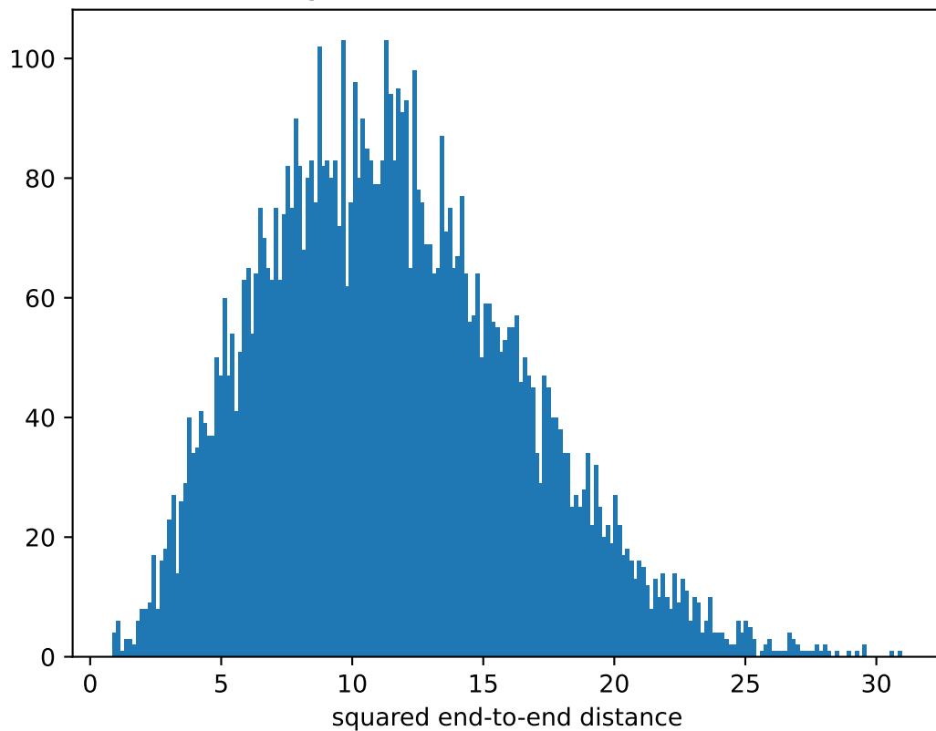
End-to-end length distribution, PVA-100, \dot{T} = 10^{-5} , T = 0.8
