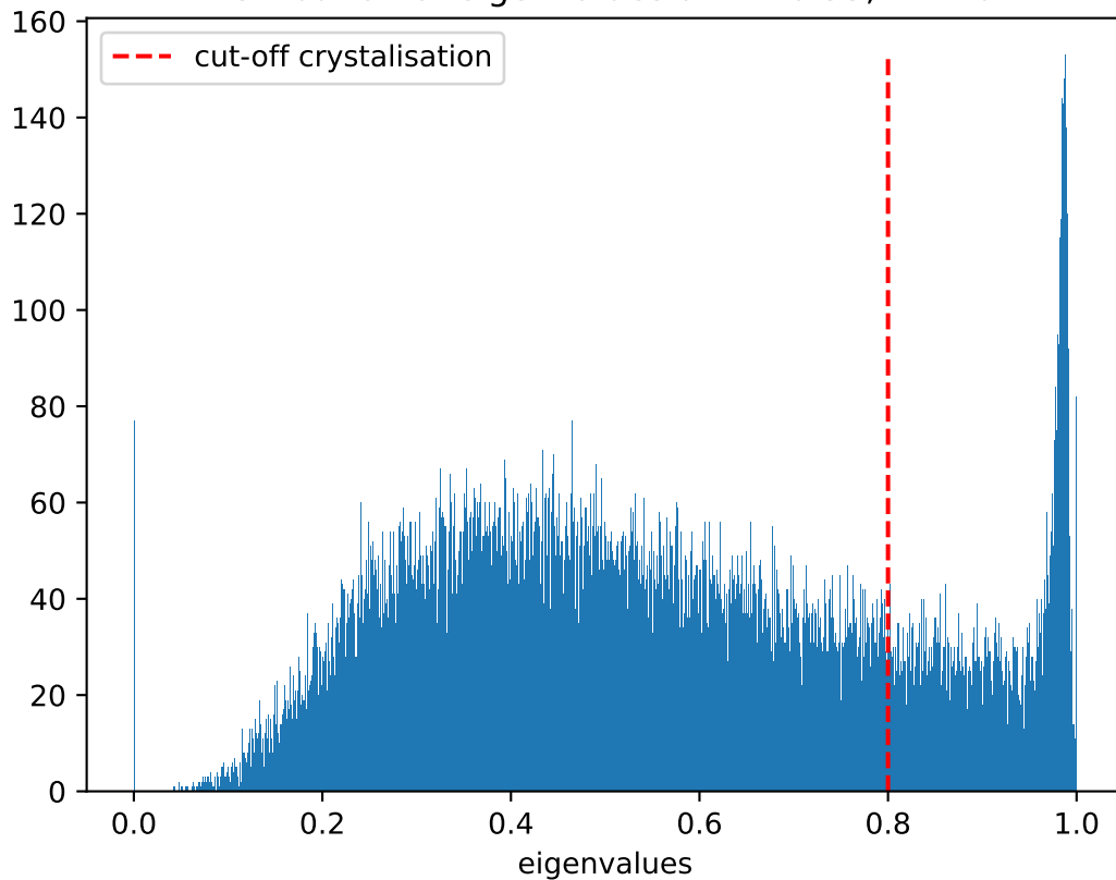
Distribution of eigenvalues at T = 0.55 , \dot{T} = 10^7
