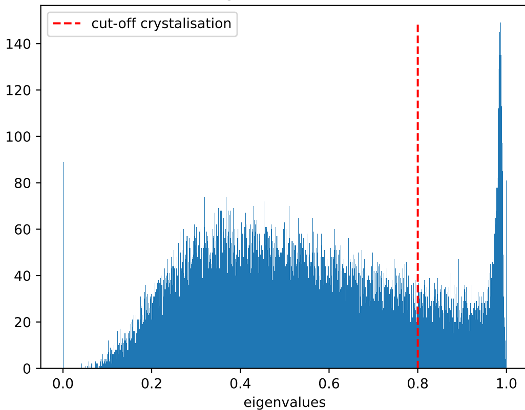
Distribution of eigenvalues at T = 0.575 , \dot{T} = 10^7
