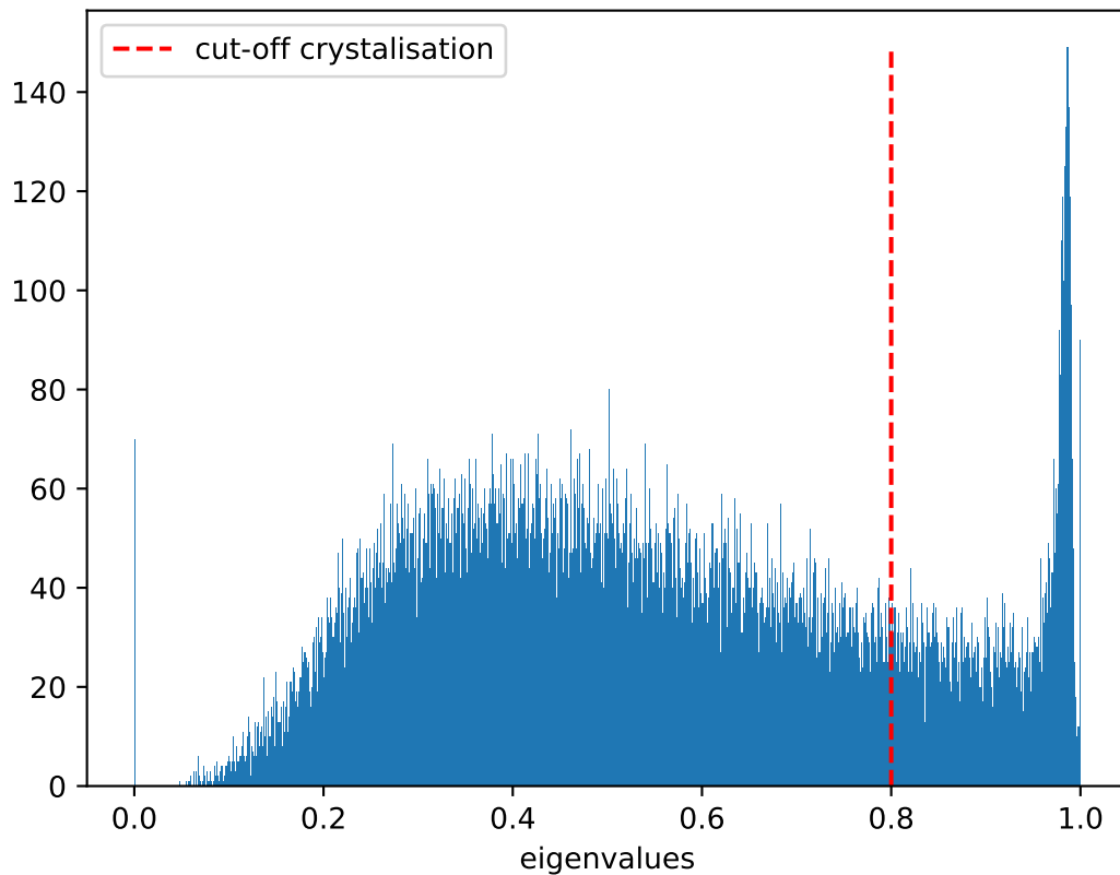
Distribution of eigenvalues at T = 0.6 , \dot{T} = 10^7
