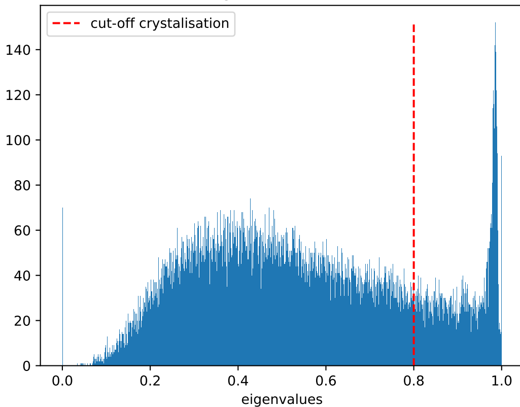
Distribution of eigenvalues at T = 0.625 , \dot{T} = 10^7
