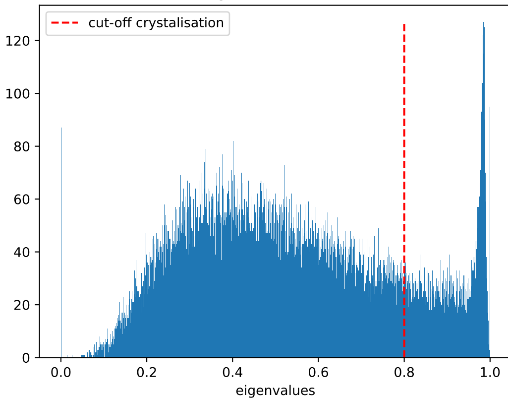
Distribution of eigenvalues at T = 0.675 , \dot{T} = 10^7
