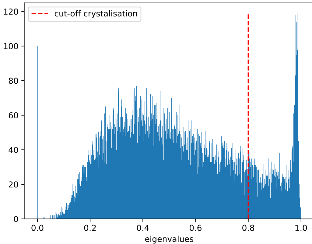
Distribution of eigenvalues at T = 0.7 , \dot{T} = 10^7
