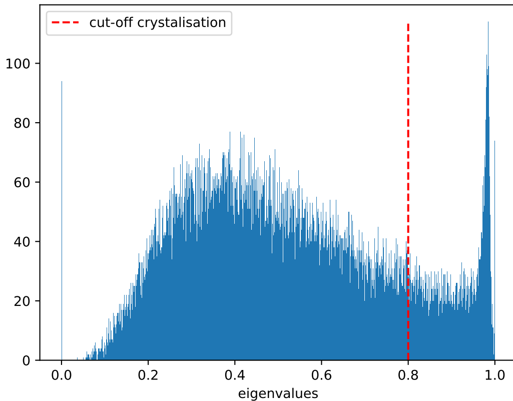
Distribution of eigenvalues at T = 0.725 , \dot{T} = 10^7
