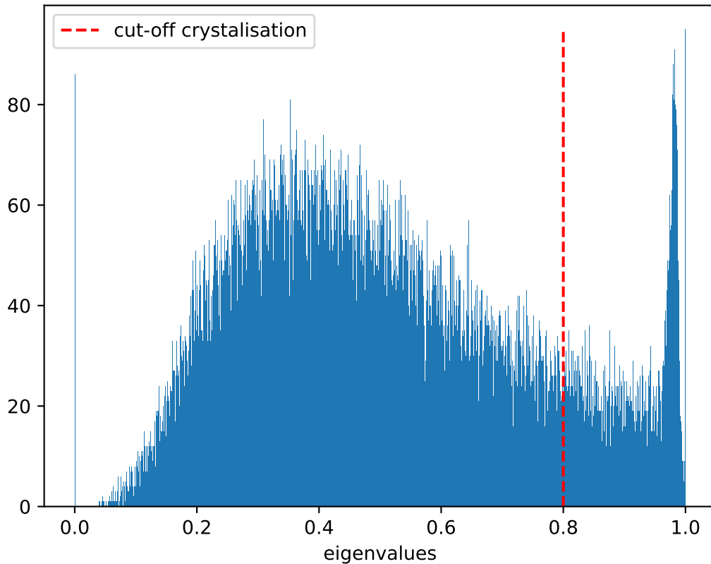
Distribution of eigenvalues at T = 0.75 , \dot{T} = 10^7
