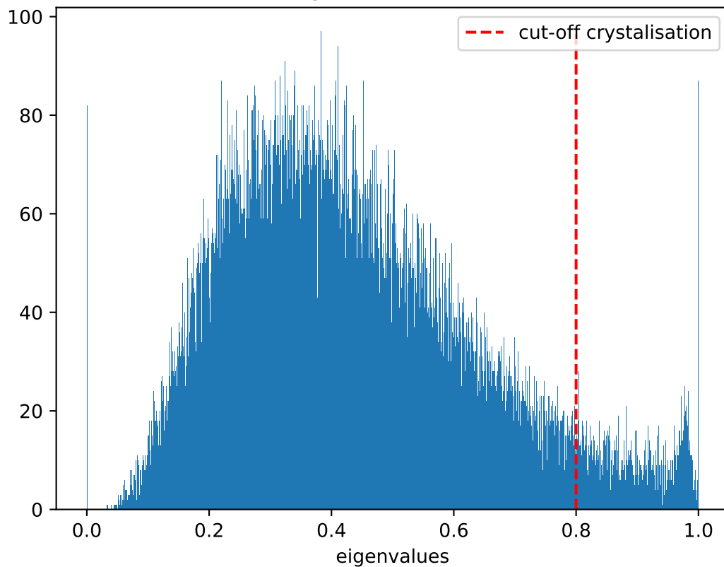
Distribution of eigenvalues at T = 0.825 , \dot{T} = 10^7
