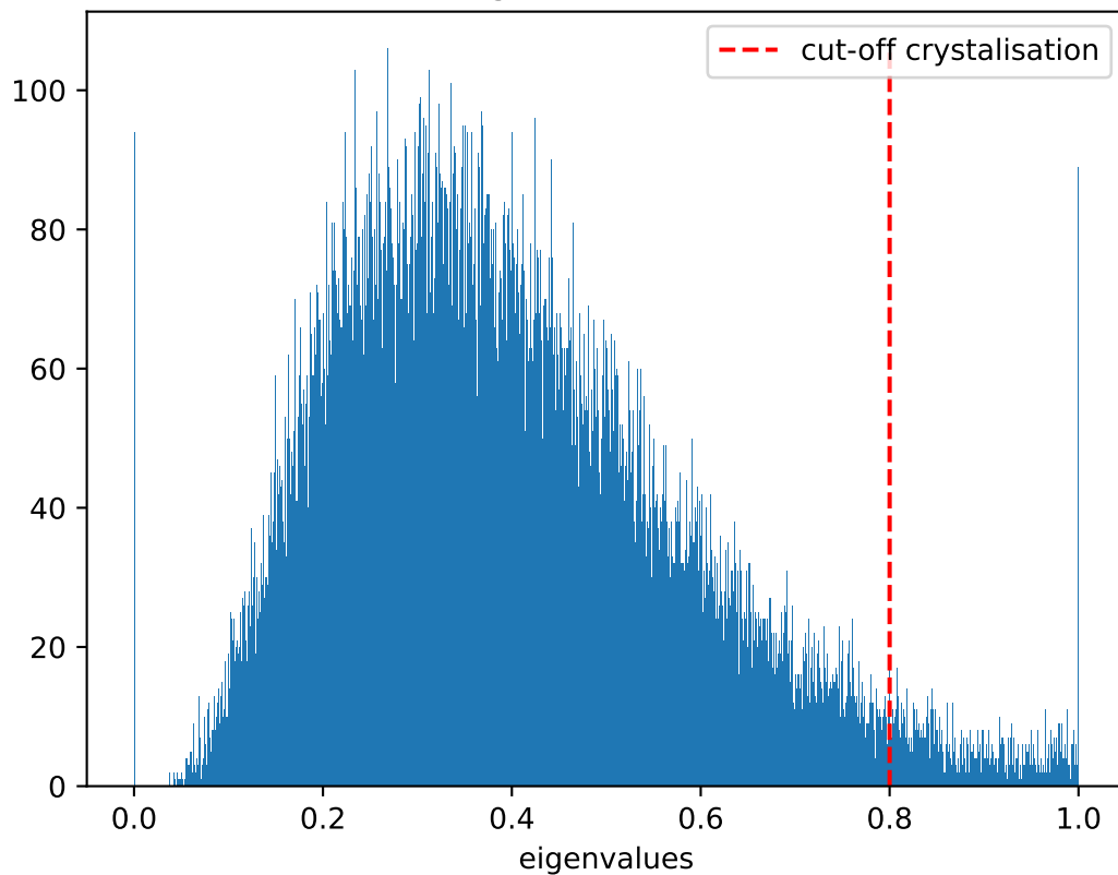
Distribution of eigenvalues at T = 0.85 , \dot{T} = 10^7
