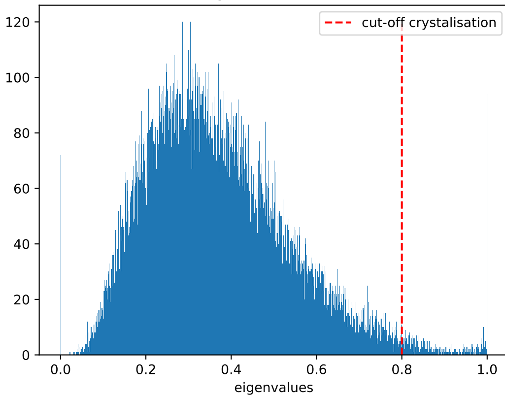
Distribution of eigenvalues at T = 0.875 , \dot{T} = 10^7
