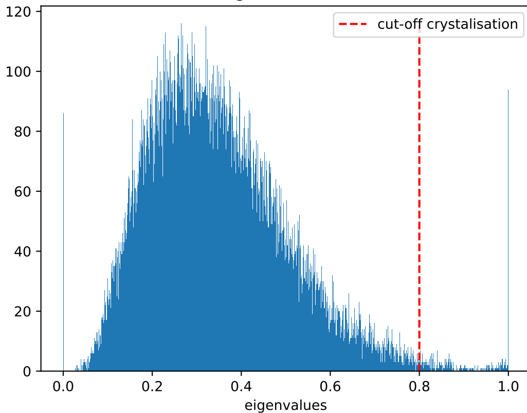
Distribution of eigenvalues at T = 0.9 , \dot{T} = 10^7
