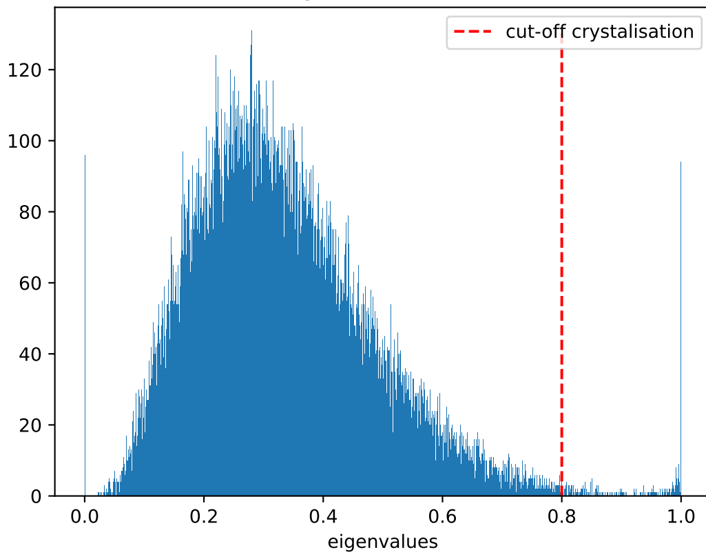
Distribution of eigenvalues at T = 0.925 , \dot{T} = 10^7
