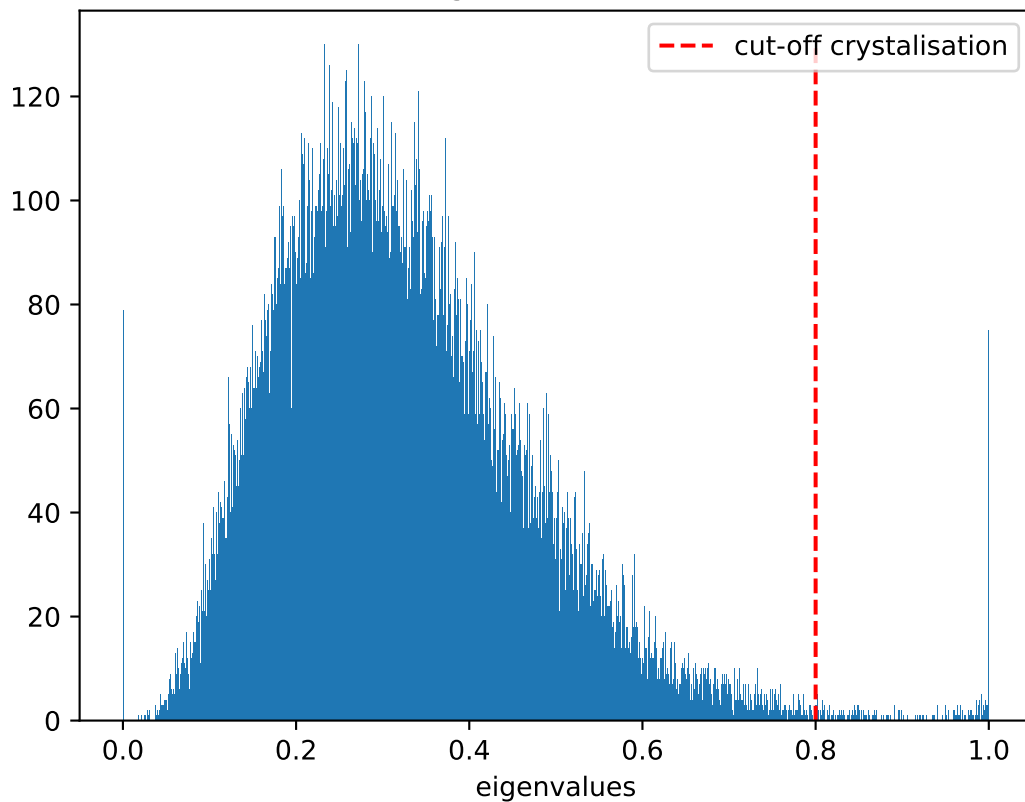
Distribution of eigenvalues at T = 0.95 , \dot{T} = 10^7
