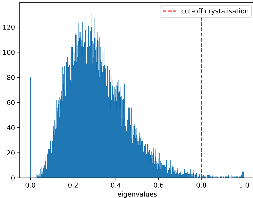
Distribution of eigenvalues at T = 0.975 , \dot{T} = 10^7
