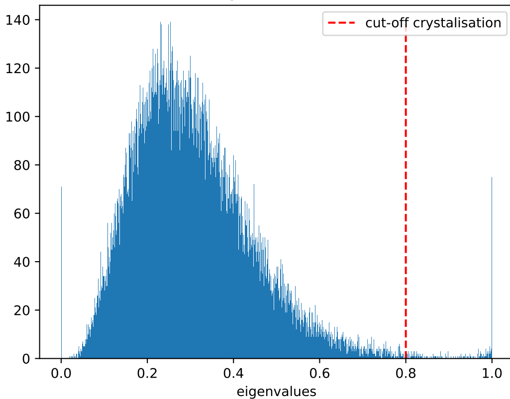
Distribution of eigenvalues at T = 1.0 , \dot{T} = 10^7
