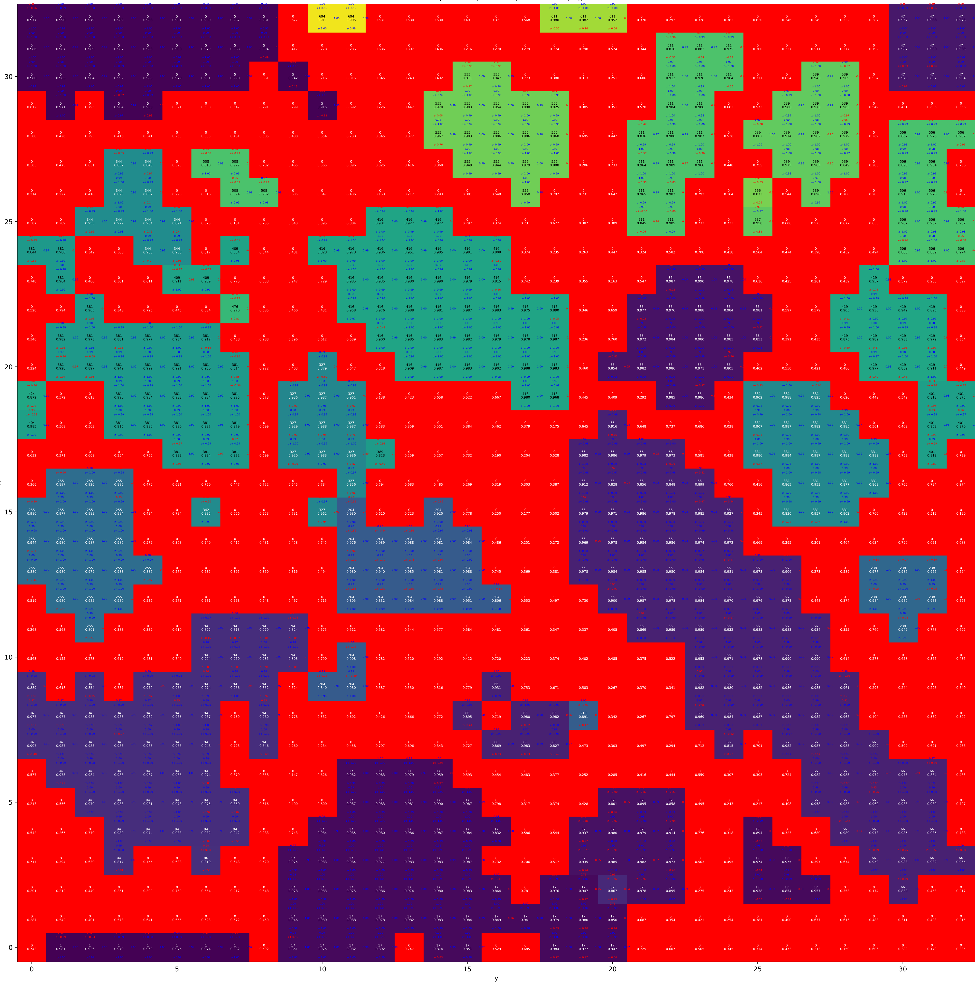
Cluster labels, PVA-100, T = 0.88, Tdot = 10**(-3), z = 2
