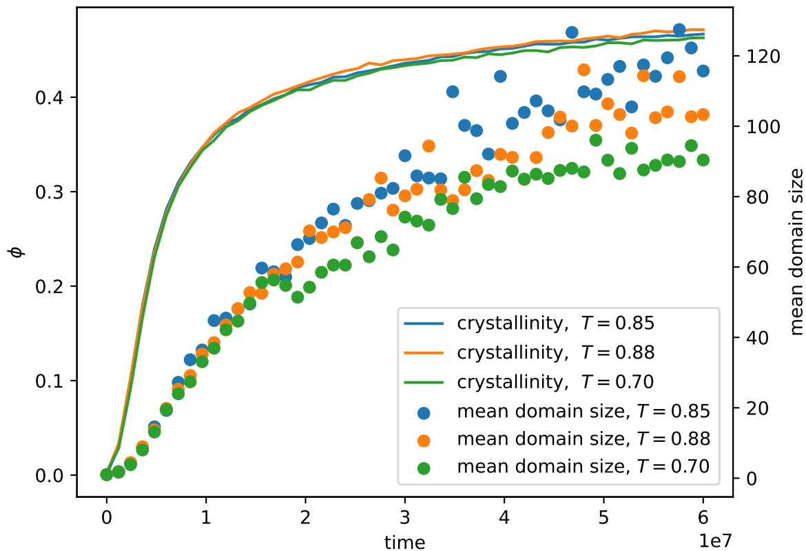
Crystallinity and mean domain size, \dot{T} = 10^{-4}
