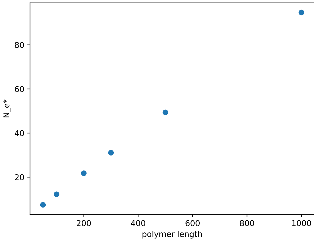
Entanglement lengths
