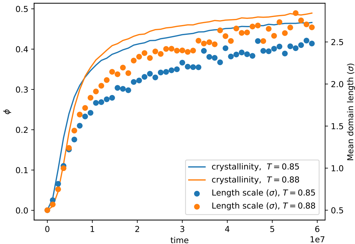
Crystallinity and mean domain size, \dot{T} = 10^{-3}
