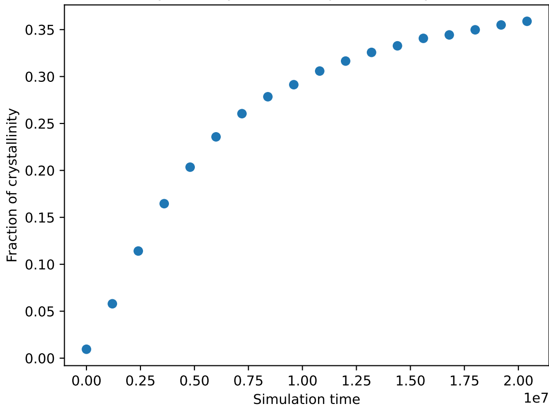
Crystallinity vs time, equilibrated system
