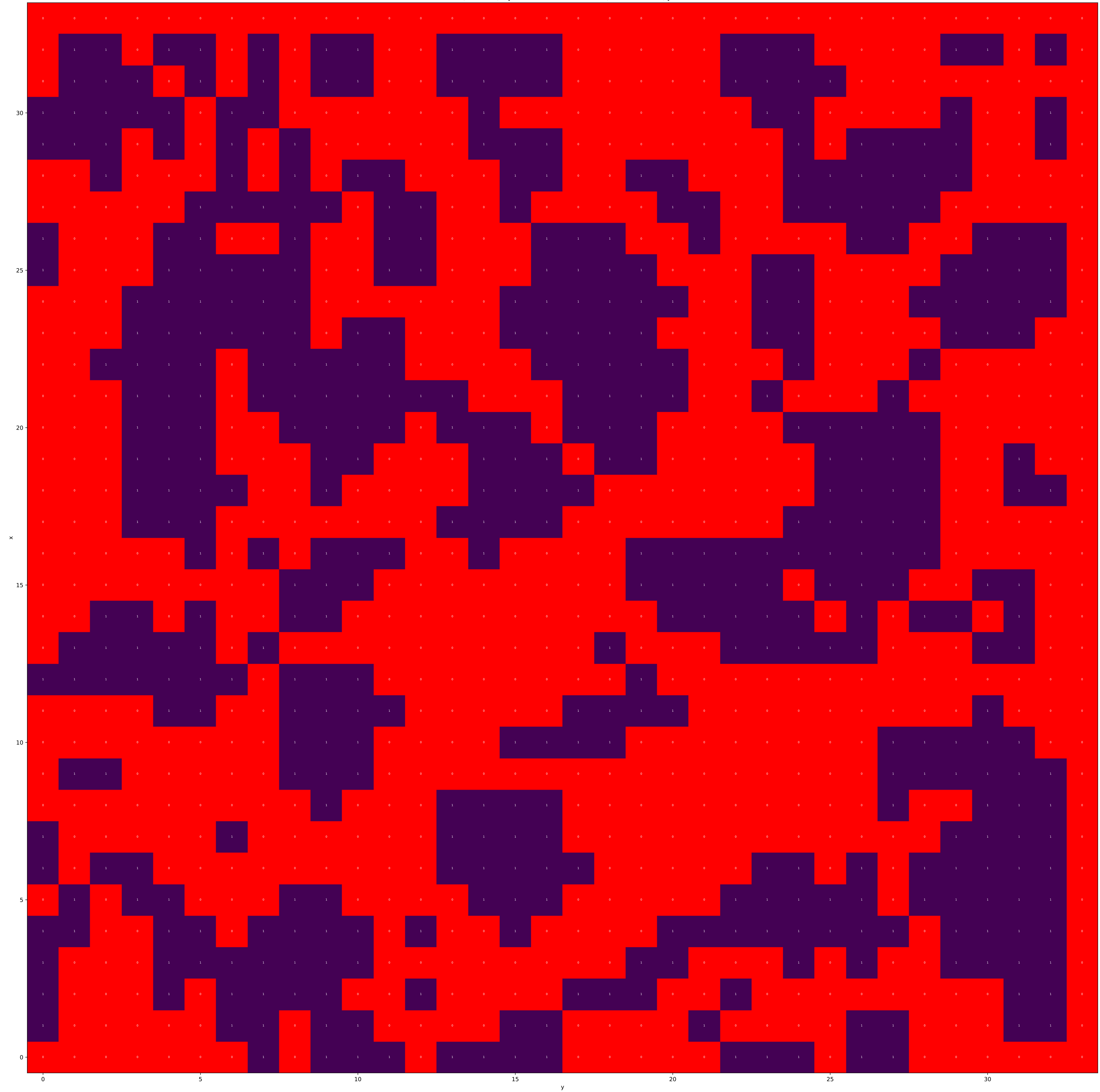
PVA-100, T = 0.88 , crystallisation via nematic20cc, xz crosssection, y = 15
