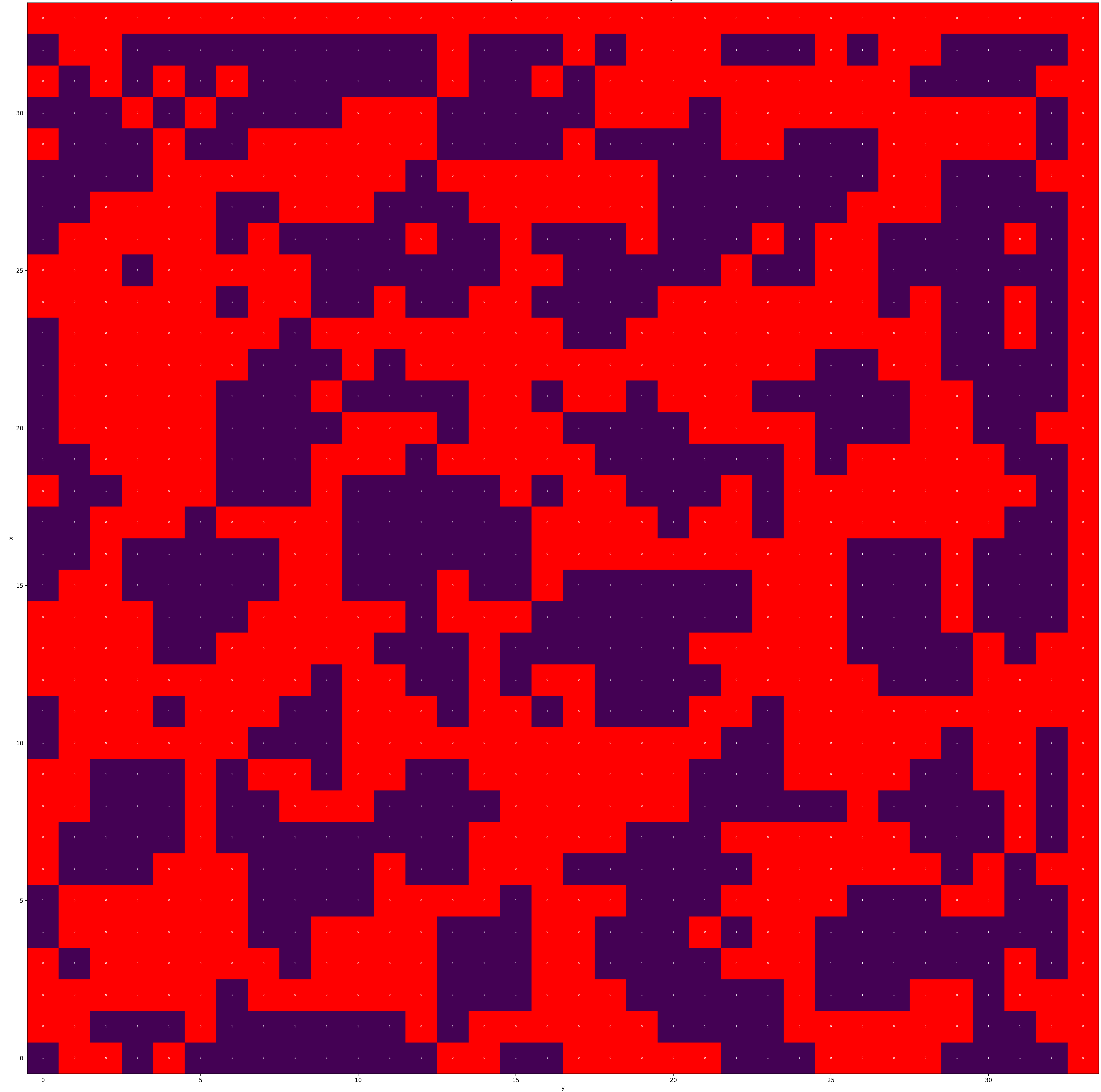
PVA-100, T = 0.88 , crystallisation via nematic20cc, xz crosssection, y = 3
