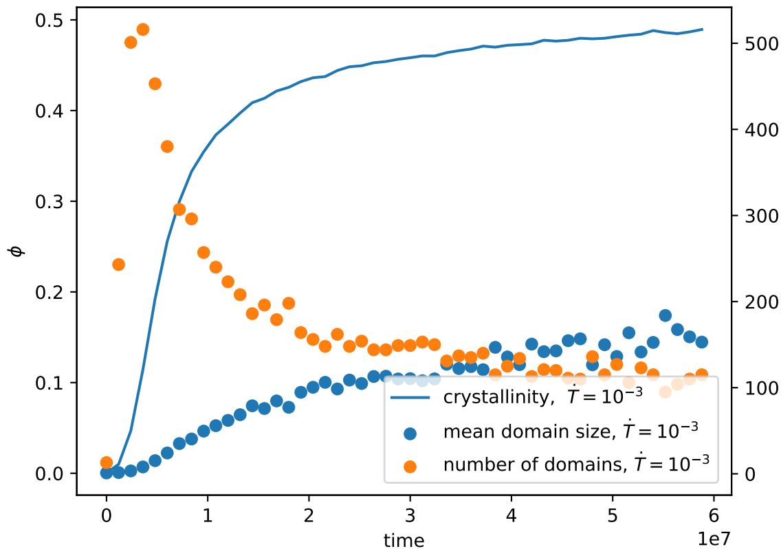
Crystallinity and mean domain size, T = 0.88
