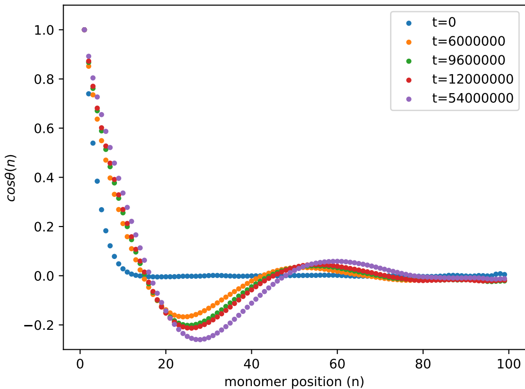
Bond-bond correlation, PVA-100, T = 0.85 , \dot{T} = 10^{-3.0}
