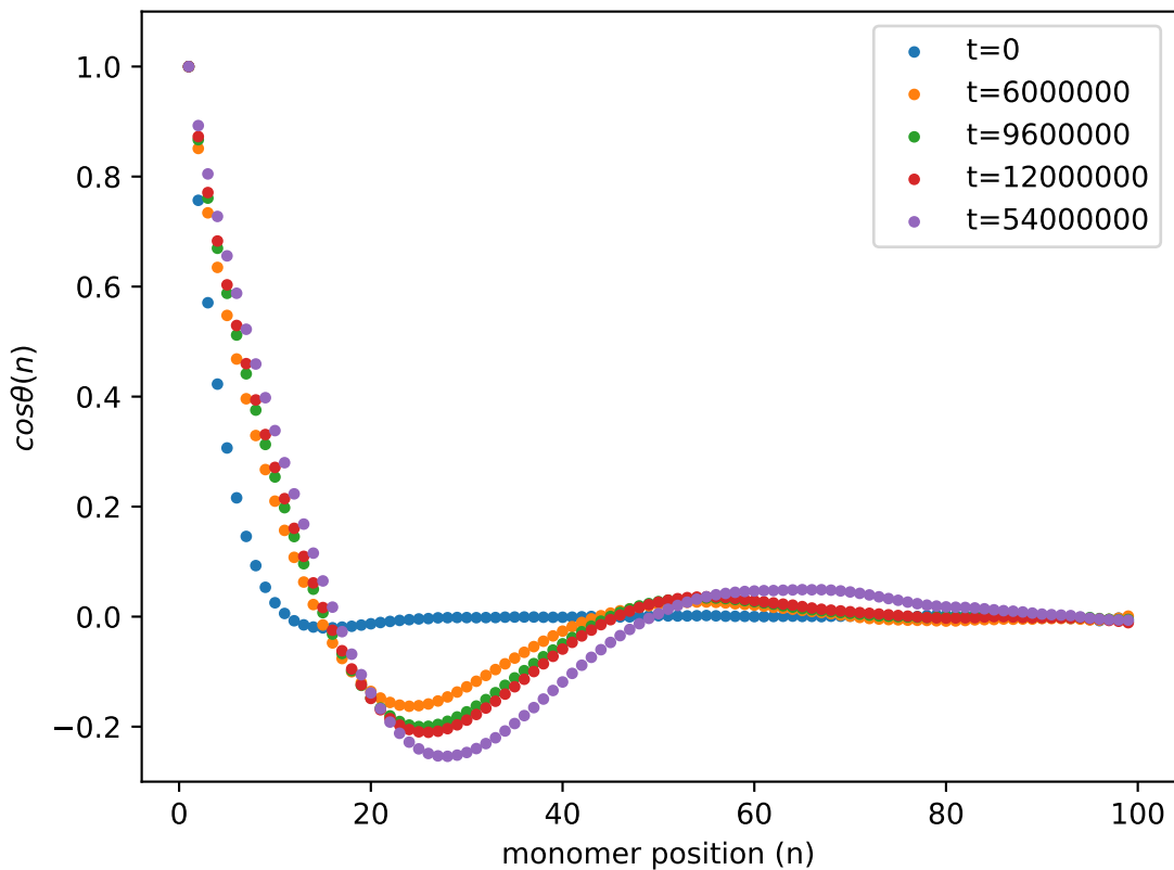
Bond-bond correlation, PVA-100, T = 0.85 , \dot{T} = 10^{-4.0}
