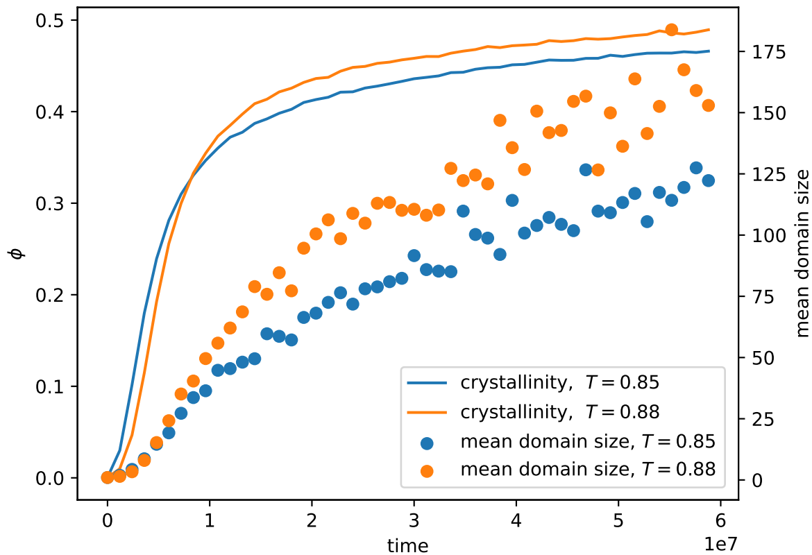
Crystallinity and mean domain size, \dot{T} = 10^{-3}
